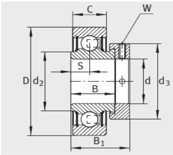
RA..-NPP、RAL..-NPP
