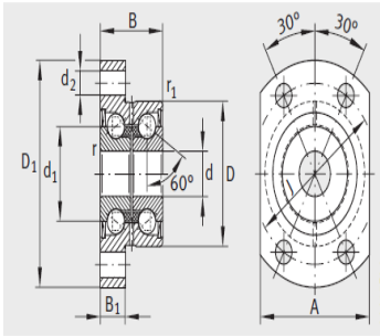
ZKLFA...2RS, ZKLFA...2Z
